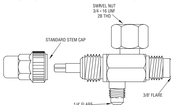
Rotalock Valve
